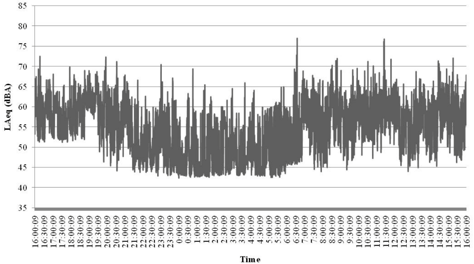
Figure 3.10. L_{Aeq} for each 10-second interval measured in Clarkson Tower 5 at the nurses' station.
