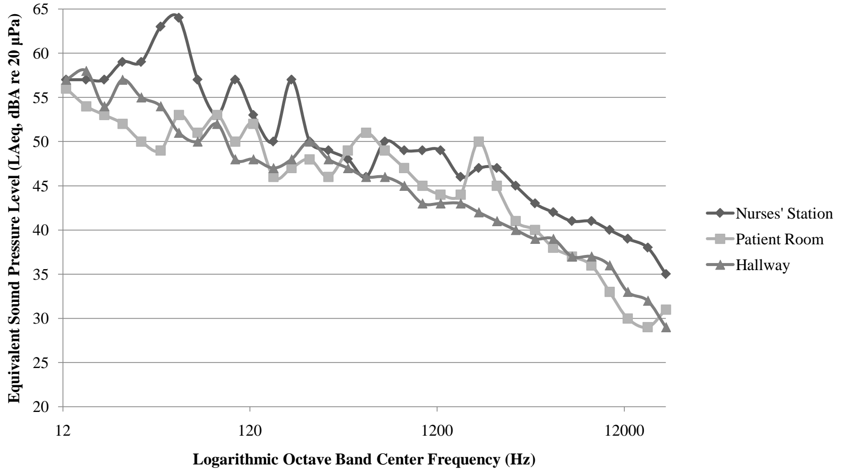
Figure 5.14. Spectral plot for all three locations from the after renovation period.
