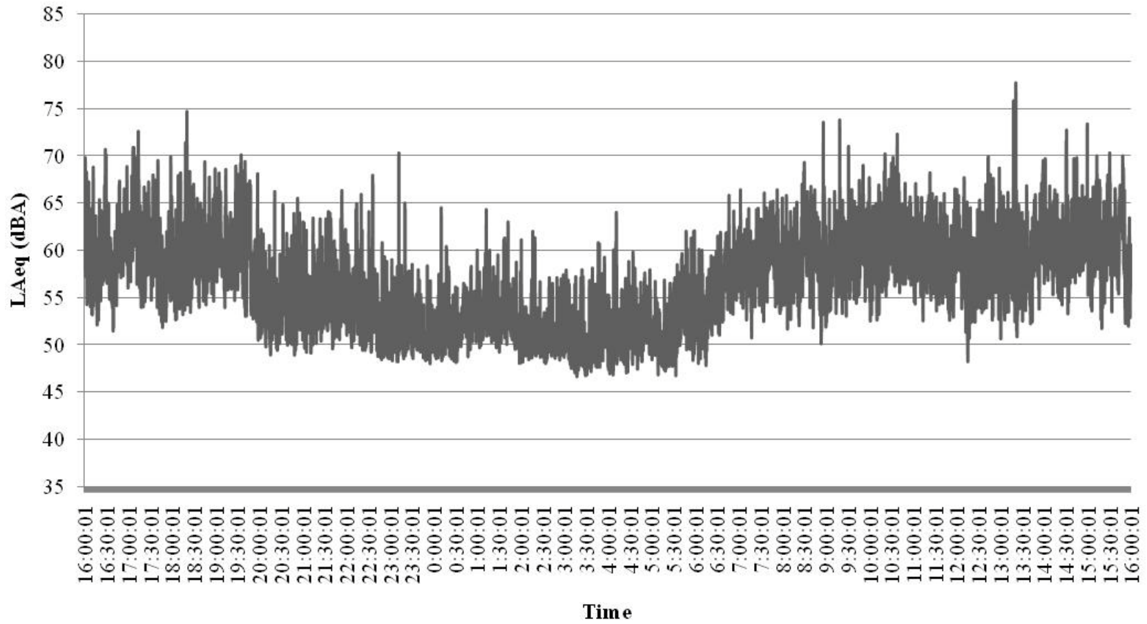
Figure 3.6. L_{Aeq} for each 10-second interval measured in University Tower 5 at the nurses' station.
