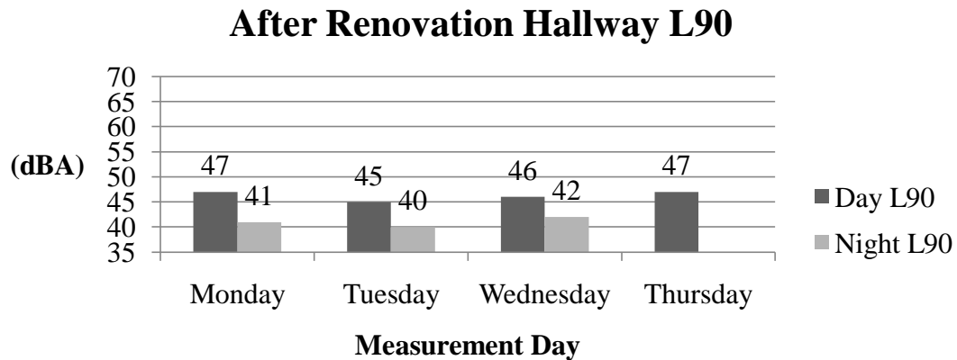
Figure 5.11. A comparison of values for percentage of exceedence over a certain level, L_{90} , for the hallway (a) before, (b) during, and (c) after renovations.
